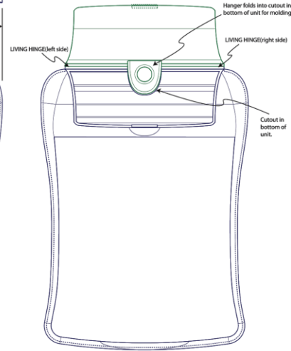
Control Drawing
